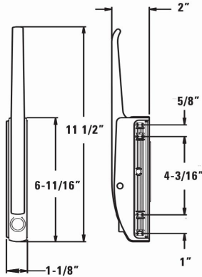
171 STRAIGHT DIE-CAST OR COMPOSITE HANDLE
