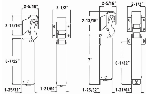
CONCEALED MOUNTING
