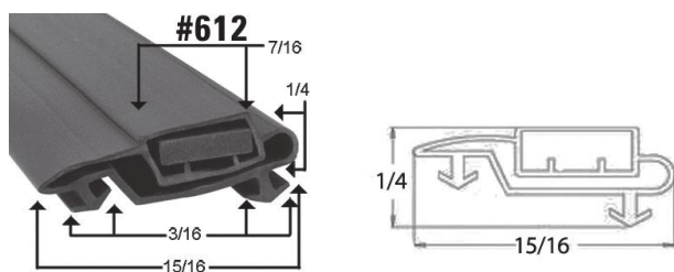
Model 1000 on Equipment Made Prior to November 1981
